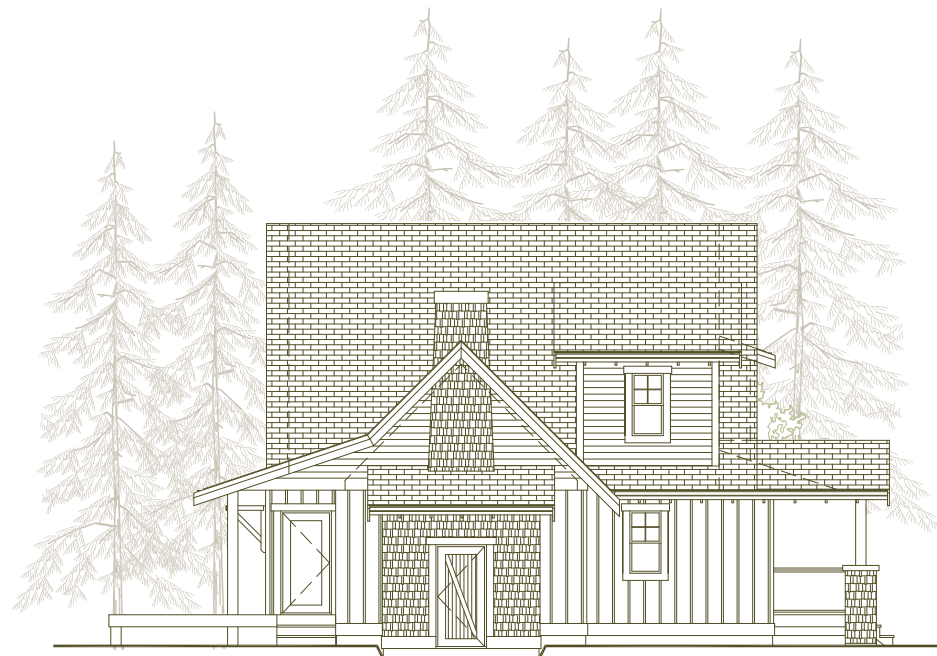
Left Elevation
